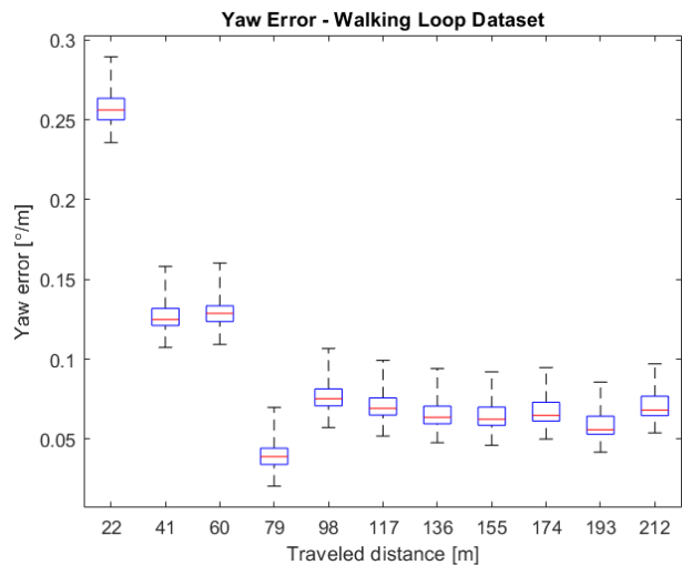
Figure 13. Yaw error for the Walking Loop Dataset.
