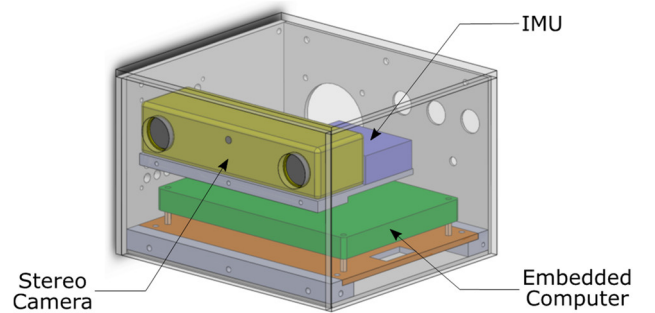
Figure 4. Visualization of the developed visual-inertial system.
