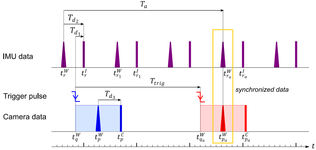
Figure 1. Time synchronization scheme between IMU and camera. Vertical bars mark the timestamps when data is received. Triangles show the true timestamps when the sensors capture the world. Trigger pulses are visualized by falling edges. Blue indicates the original trigger signal and camera data with exposure delay, while red shows the synchronized ones. IMU data is colored purple. The yellow rectangle marks a synchronized IMU-camera data pair.
