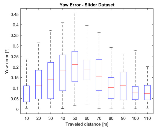
Figure 9. Error statistics of yaw error for the Slider Dataset.
