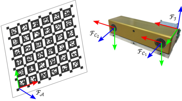
Figure 2. Coordinate frames of visual inertial sensors and calibration pattern. The calibration pattern is formed by AprilTag [14].
