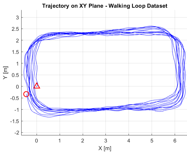
Figure 10. The trajectory of VIO system plotted on XY plane, for the Walking Loop Dataset. The red triangle and circle mark the beginning and end point of the trajectory, respectively.
