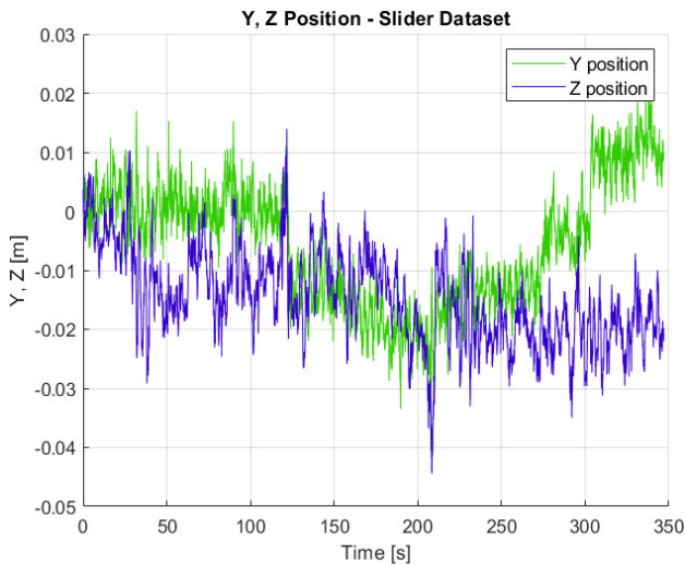
Figure 7. Estimated Y and Z position maintained around zero for the Slider Dataset.
