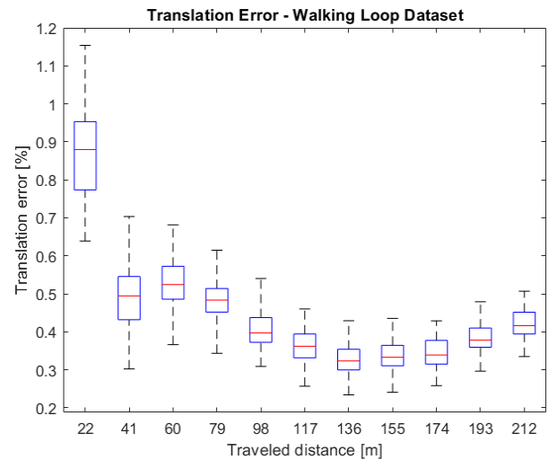
Figure 12. Translation error for the Walking Loop Dataset.
