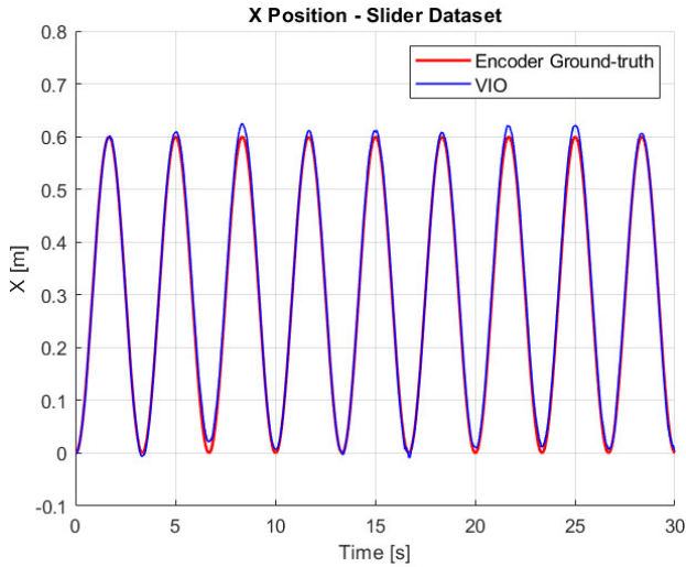
Figure 6. Estimated X position in comparison with encoder ground-truth for the Slider Dataset.
